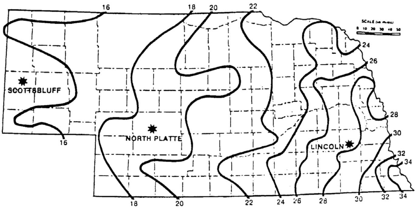
FIG 18.4 Figure 18.2 Average Annual Precipitation, Inches
