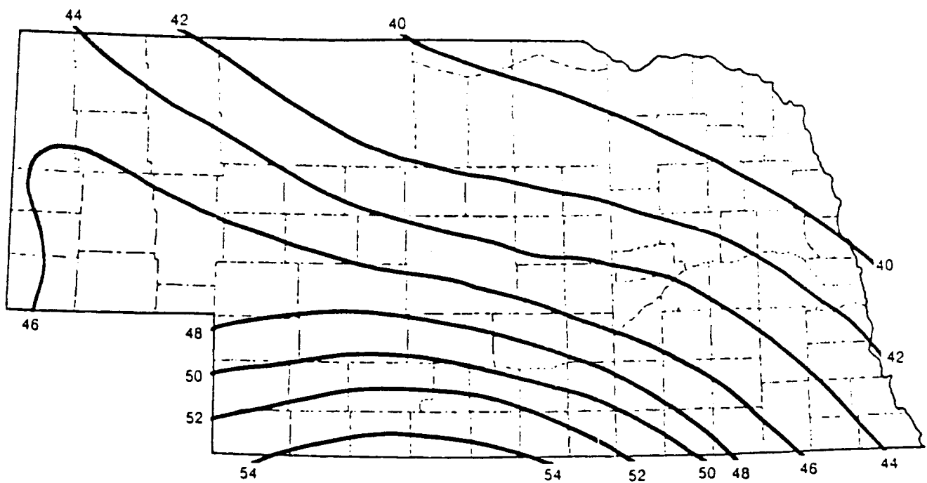
FIG 18.3 Figure 18.1 Average Annual Lake Evaporation, Inches
